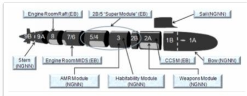
Figure 55. Virginia Class Submarine Built Using Modular Construction Practices
