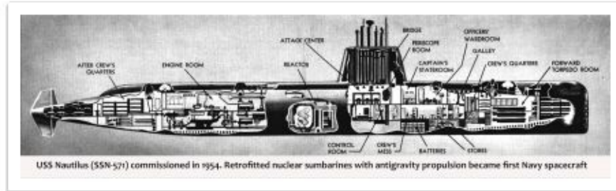
Figure 48. First "Nautilus Class" Nuclear Submarine Built for US Navy by General Dynamics
