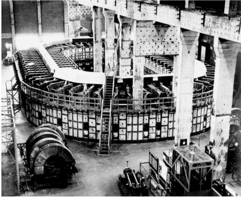
One of E.O. Lawrence's Beta Calutrons Uranium Enrichment Cyclotrons at Oak Ridge, Tennessee, during World War Two
