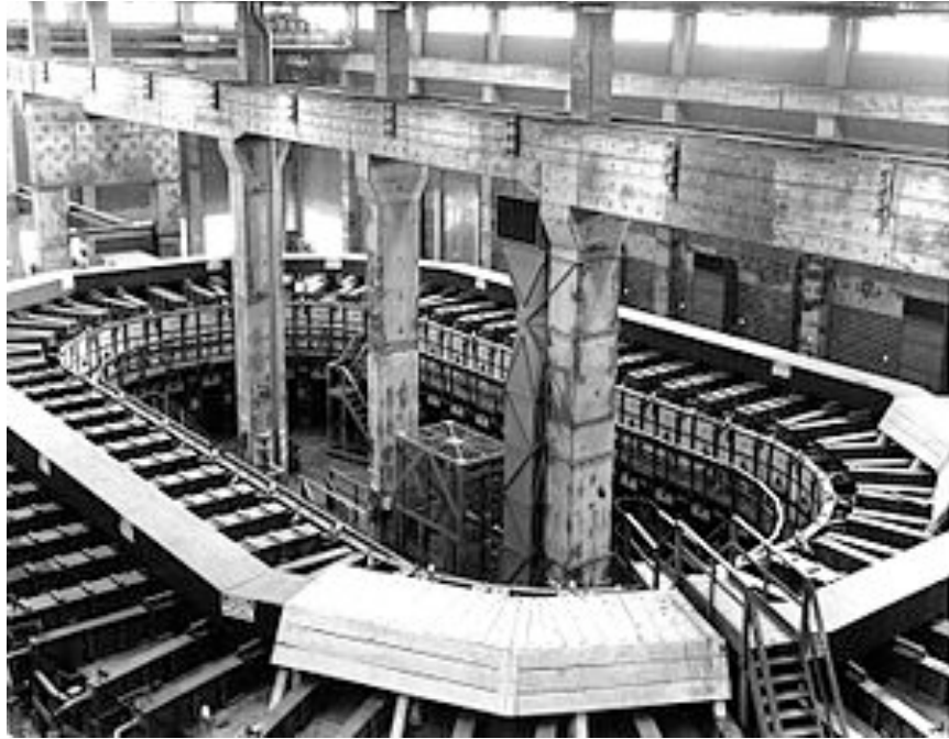
Another view of one of Lawrence's Beta Calutron Uranium Enrichment Cyclotrons at Oak Ridge, Tennessee
