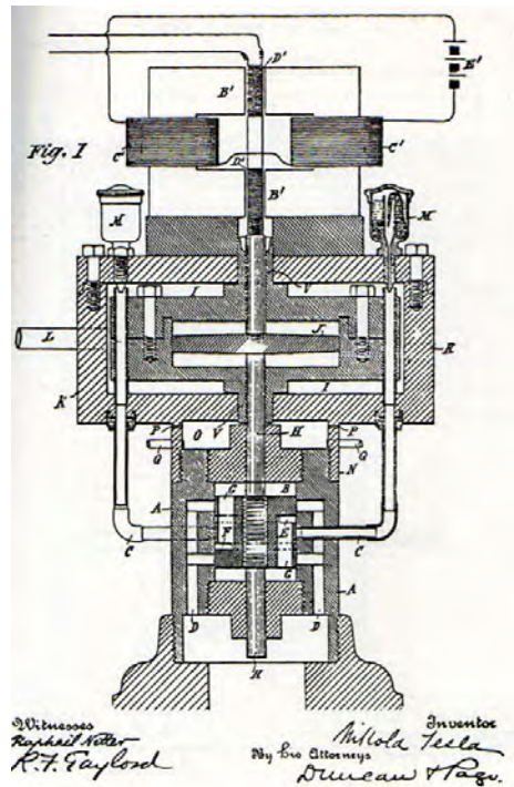
Nicola Tesla U.S. Patent 511,916, Jan 2 1894, for an "Electrical Generator," really an Electro-Mechanical Oscillator 23
